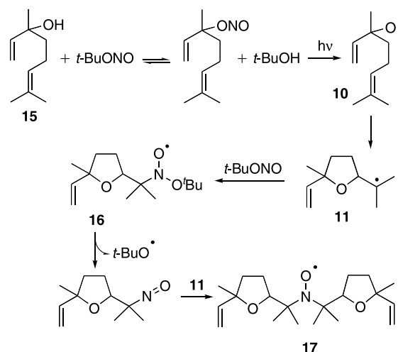
Scheme 5. Spin trapping of alkyl radicals derived from linalool 15 .
