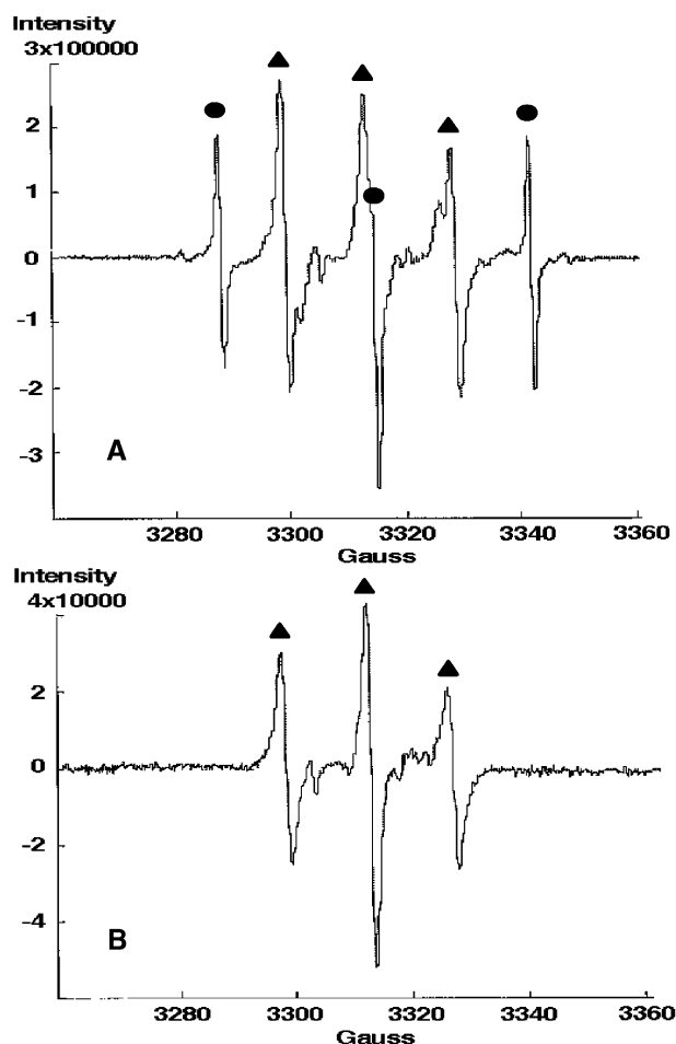
Figure 5. A) EPR spectrum obtained in the photolysis of an acetonitrile solution of 15 , 104 mM and t -BuONO, 224 mM, at 240 K (flow rate 1 mL/h; laser at 50 mW power), showing radicals 16 (●) and 17 (▲). (B) EPR spectrum obtained in the photolysis of an acetonitrile solution of 15 , 50 mM, and t -BuONO, 110 mM, at 240 K (flow rate 2 mL/h; laser at 5 mW power), showing radical 17 (▲).
