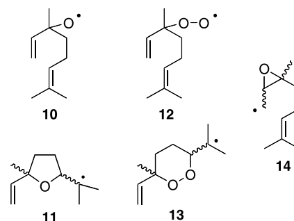
Figure 2. Radical intermediates derived from compound 1 .
