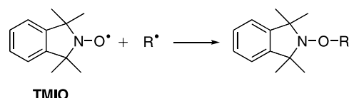
Scheme 1. Formation of alkoxyamines by radical trapping with TMIO.
