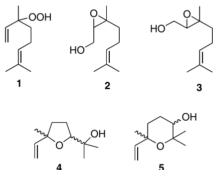
Figure 1. Potential rearrangement compounds from linalyl hydroperoxide.
