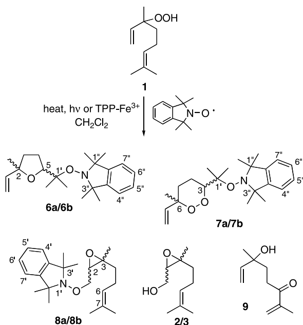
Scheme 2. Trapping of radicals derived from linalyl hydroperoxide 1 .
