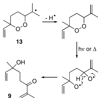
Scheme 4. Mechanism suggested for the obtention of 9 .
