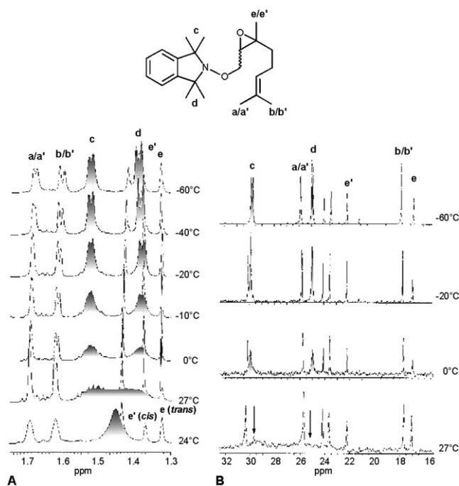
Figure 4. Identification of methyl groups in the mixture of diastereomers 8a/b by ^1\text{H} (A) and ^{13}\text{C} NMR (B) at different temperatures.
